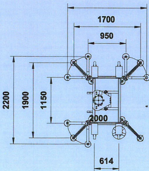
Dimensioni base Base frame dimensions
